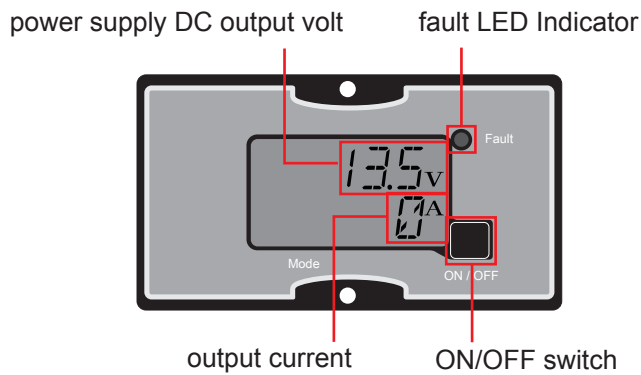
5. Mode 2: power supply mode.
